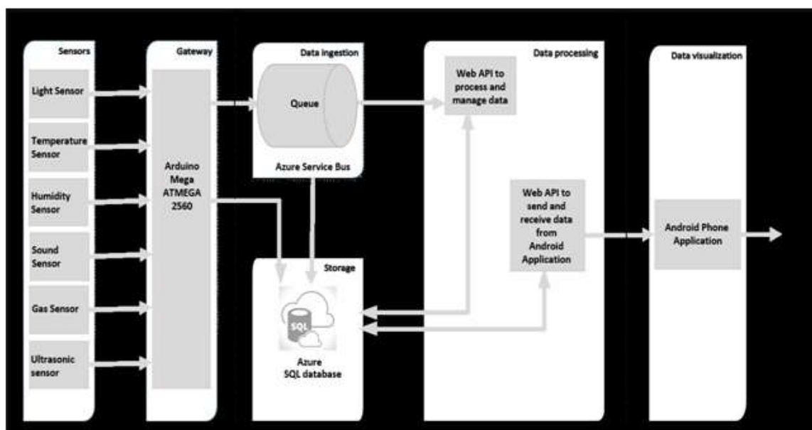
Figure 1 Architectural of Home Environment Monitoring System
